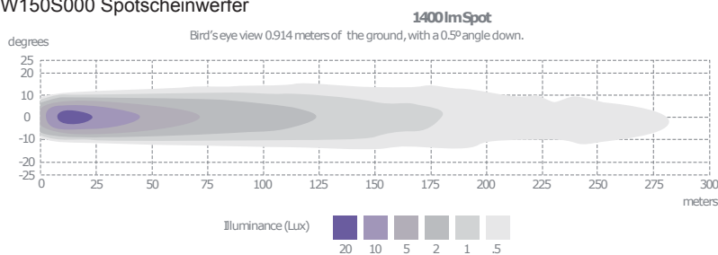
W150S000 Spotscheinwerfer
